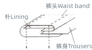
裤头Waist band 补Lining 裤身Trousers
